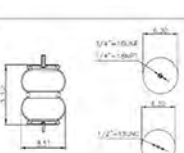
Air Spring - Double Bellows - Watson/Ridewell
