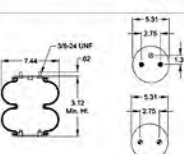
Air Spring - Double Convoluted - Hendrickson
